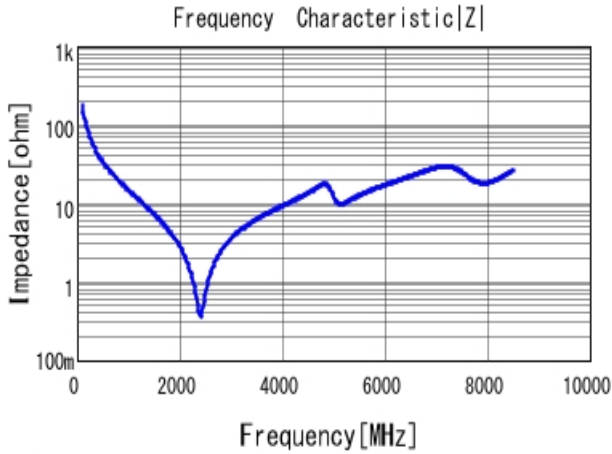
■ GRM1885C1H9R0BA01 |Z| DCOV, 25degC
