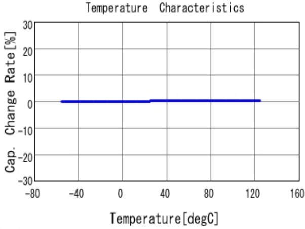
■ GRM1885C1H8R2DA01 C-Temp. capchange, DCOV, AC1Vrms
