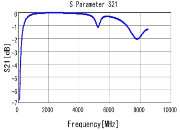
■ GRM1885C1H8R2DA01 S21 DCOV, 25degC
