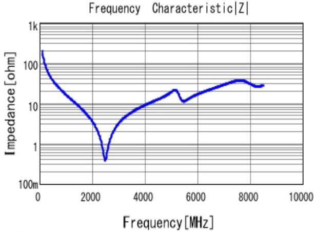
■ GRM1885C1H8R2DA01 |Z| DCOV, 25degC
