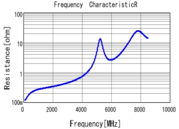
■ GRM1885C1H8R2DA01 R DCOV, 25degC
