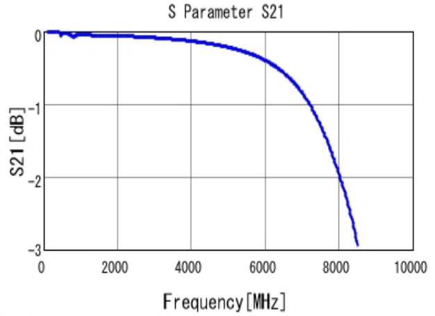
■ GRM1885C1H821JA01 S21 DCOV, 25degC
