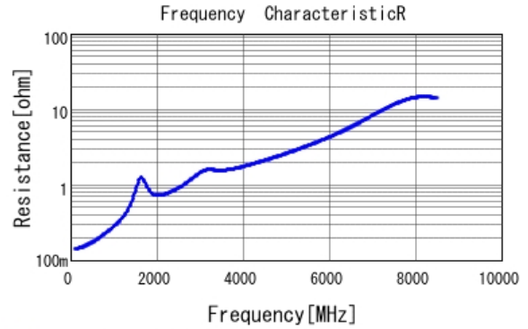
■ GRM1885C1H820JA01 R DCOV, 25degC
