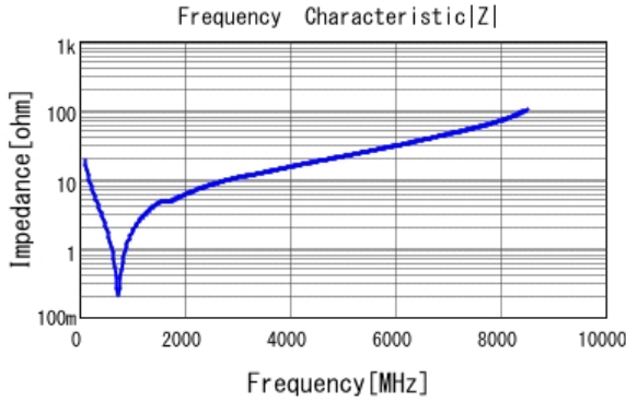
■ GRM1885C1H820JA01 |Z| DCOV, 25degC
