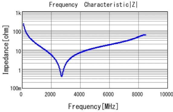
■ GRM1885C1H6R8DA01 |Z| DCOV, 25degC
