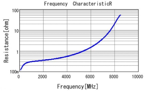
■ GRM1885C1H6R8CA01 R DCOV, 25degC
