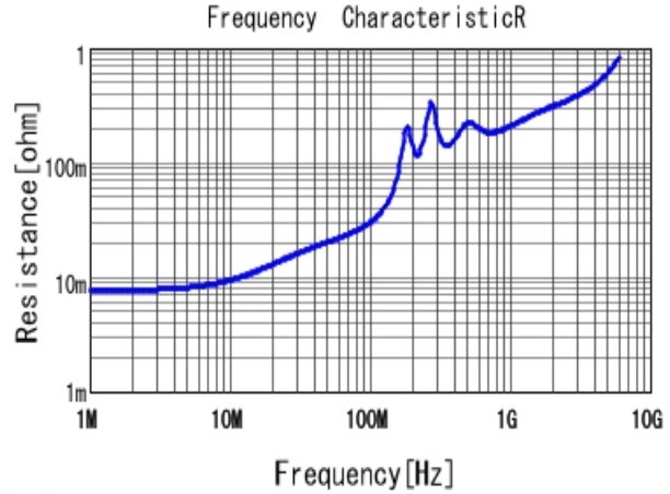
■ GRM1885C1H682JA01 R DCOV, 25degC
