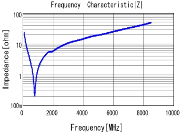
■ GRM1885C1H680JA01 |Z| DCOV, 25degC
