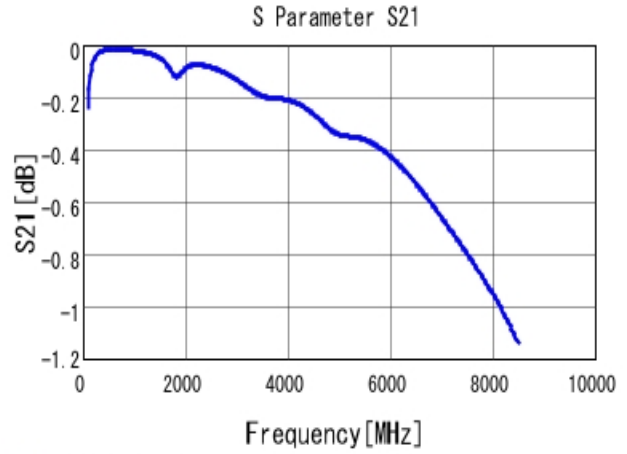
■ GRM1885C1H680JA01 S21 DCOV, 25degC
