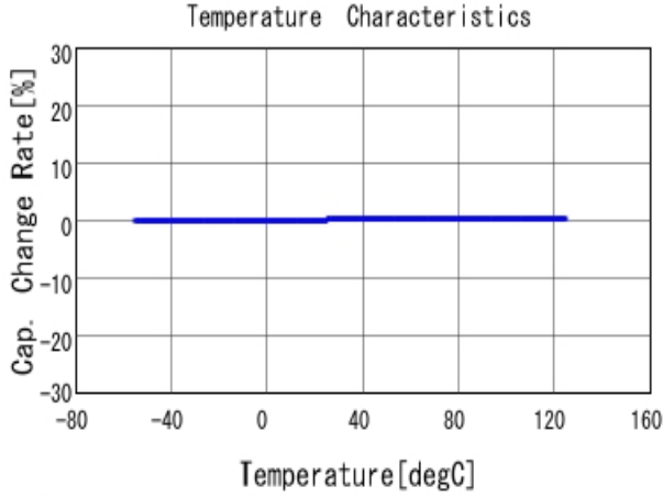
■ GRM1885C1H5R6DA01 C-Temp. capchange, DCOV, AC1Vrms
