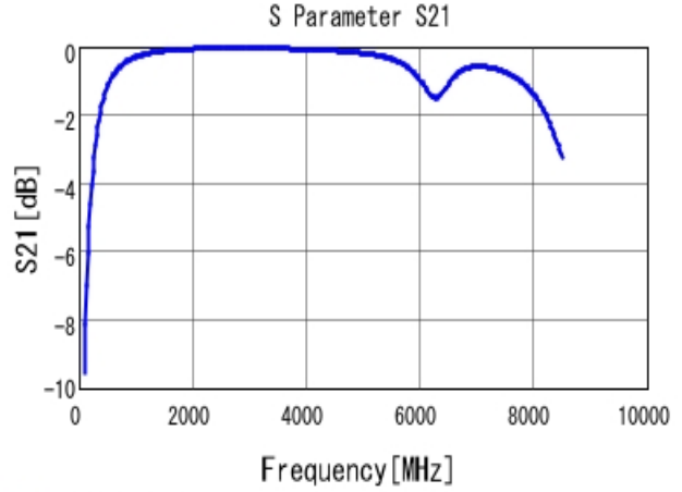
■ GRM1885C1H5R6DA01 S21 DCOV, 25degC
