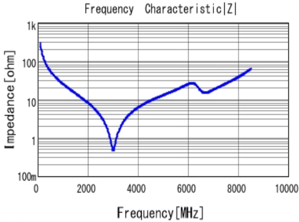
■ GRM1885C1H5R6DA01 |Z| DCOV, 25degC
