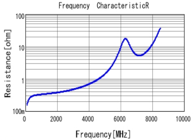
■ GRM1885C1H5R6DA01 R DCOV, 25degC
