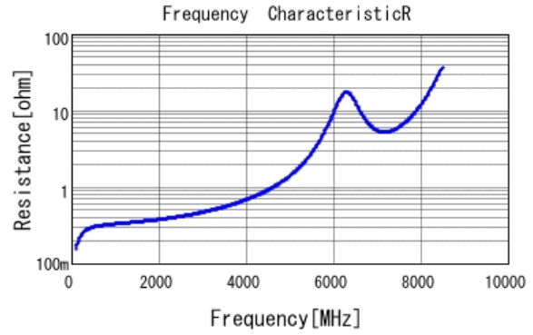
■ GRM1885C1H5R6CA01 R DCOV, 25degC
