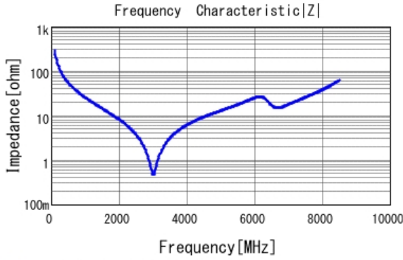
■ GRM1885C1H5R6CA01 |Z| DCOV, 25degC
