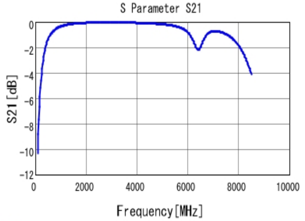
■ GRM1885C1H5R1CA01 S21 DCOV, 25degC
