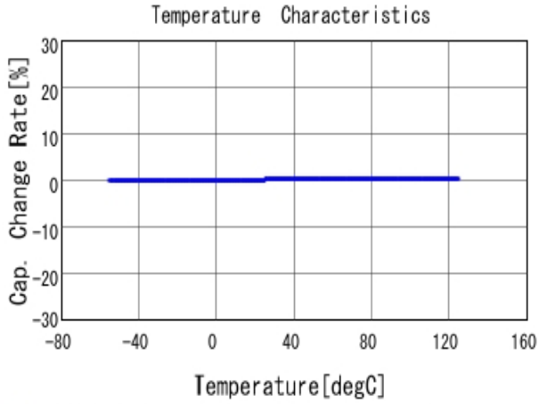
■ GRM1885C1H5R1CA01 C-Temp. capchange, DCOV, AC1Vrms
