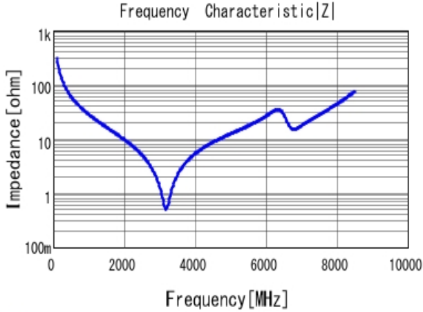
■ GRM1885C1H5R1CA01 |Z| DCOV, 25degC
