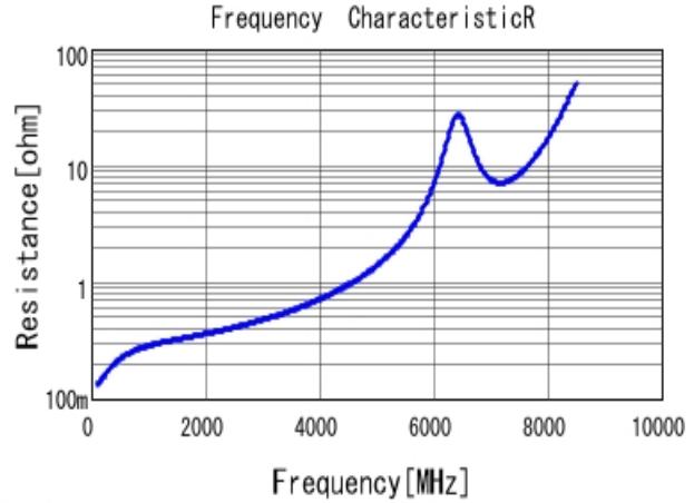
■ GRM1885C1H5R1CA01 R DCOV, 25degC
