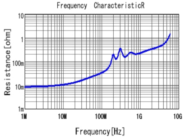
■ GRM1885C1H562JA01 R DCOV, 25degC
