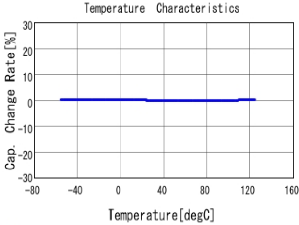
■ GRM1885C1H562JA01 C-Temp. capchange, DCOV, AC1Vrms
