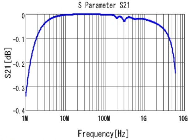
■ GRM1885C1H562JA01 S21 DCOV, 25degC
