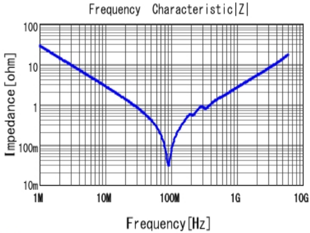
■ GRM1885C1H562JA01 |Z| DCOV, 25degC
