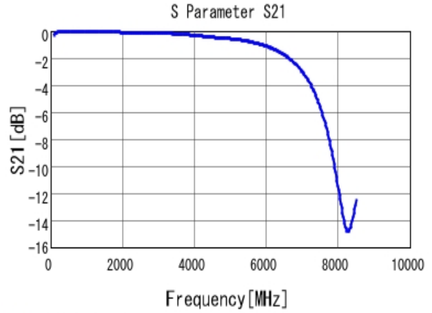
■ GRM1885C1H560JA01 S21 DCOV, 25degC
