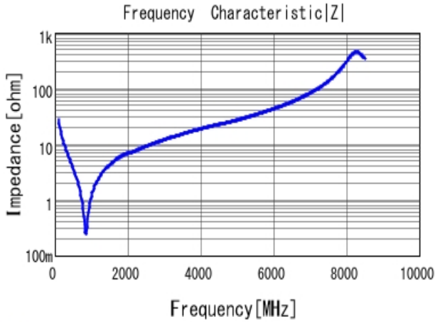
■ GRM1885C1H560JA01 |Z| DCOV, 25degC
