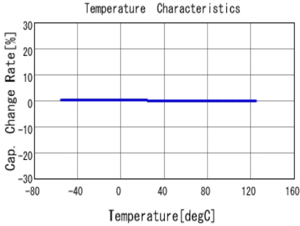
■ GRM1885C1H560JA01 C-Temp. capchange, DCOV, AC1Vrms
