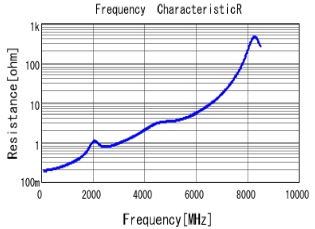
■ GRM1885C1H560JA01 R DCOV, 25degC
