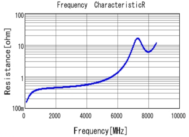
■ GRM1885C1H4R3BA01 R DCOV, 25degC
