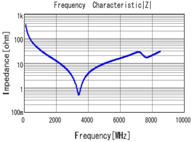
■ GRM1885C1H4R3BA01 |Z| DCOV, 25degC
