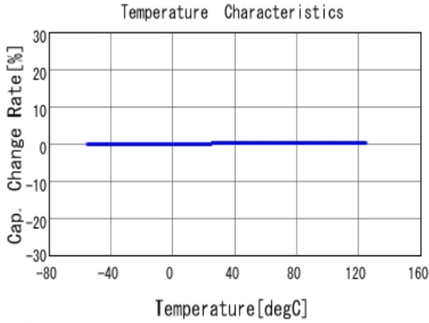
■ GRM1885C1H4R3BA01 C-Temp. capchange, DCOV, AC1Vrms
