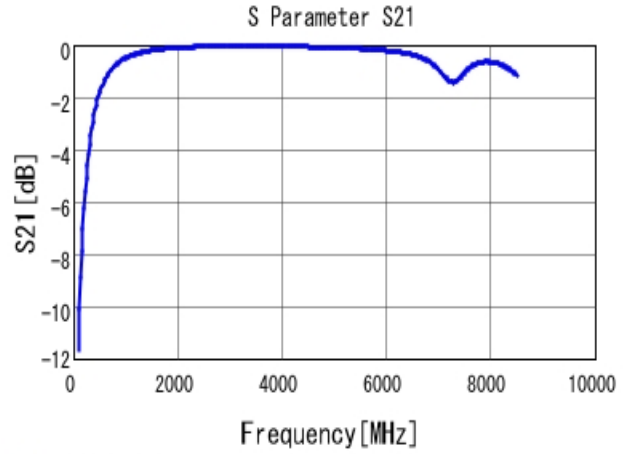
■ GRM1885C1H4R3BA01 S21 DCOV, 25degC
