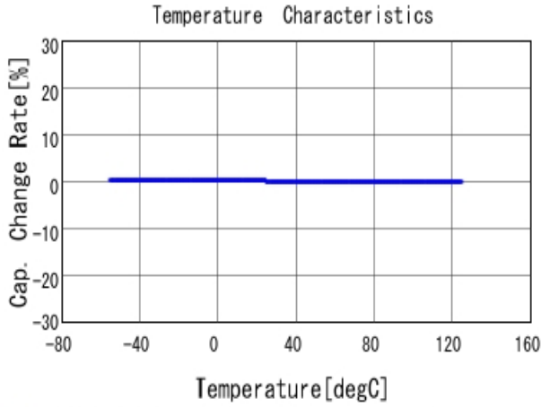
■ GRM1885C1H471JA01 C-Temp. capchange, DCOV, AC1Vrms
