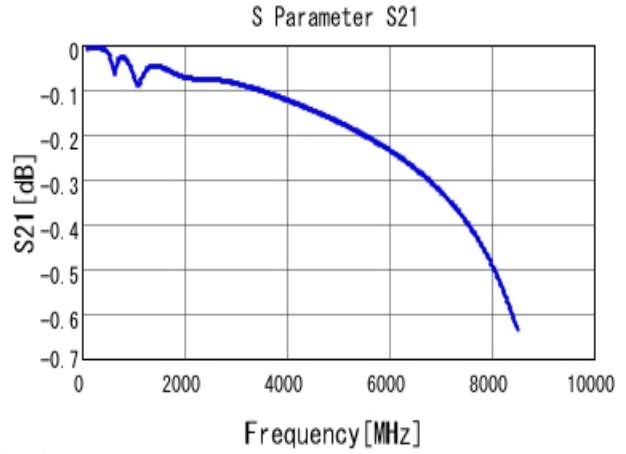
■ GRM1885C1H471JA01 S21 DCOV, 25degC
