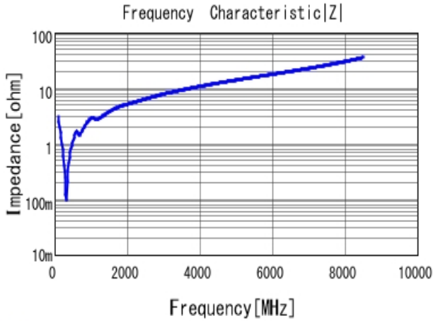
■ GRM1885C1H471JA01 |Z| DCOV, 25degC
