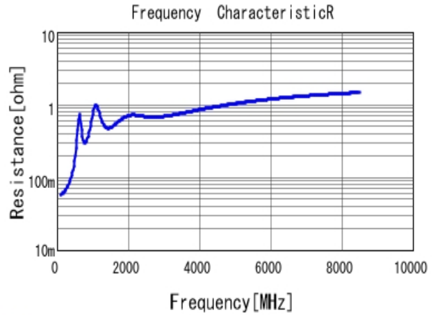
■ GRM1885C1H471JA01 R DCOV, 25degC
