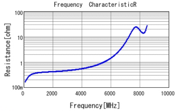
■ GRM1885C1H3R9CA01 R DCOV, 25degC
