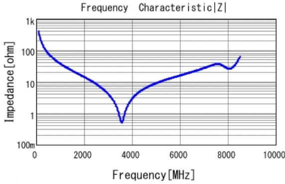
■ GRM1885C1H3R9CA01 |Z| DCOV, 25degC
