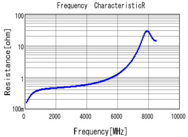
■ GRM1885C1H3R6CA01 R DCOV, 25degC
