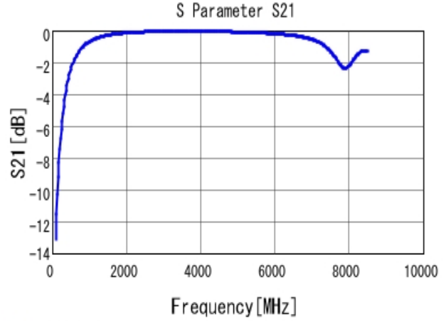
■ GRM1885C1H3R6CA01 S21 DCOV, 25degC
