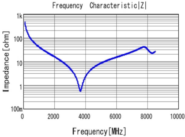
■ GRM1885C1H3R6CA01 |Z| DCOV, 25degC
