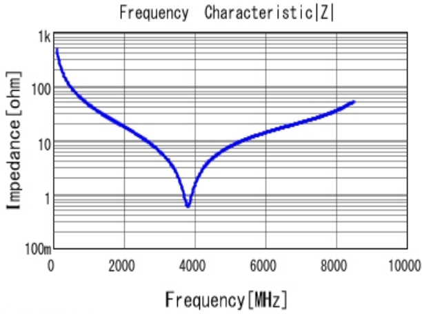
■ GRM1885C1H3R3CA01 |Z| DCOV, 25degC
