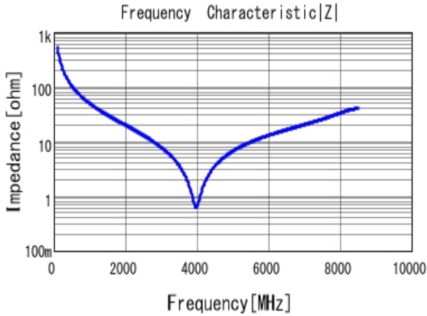
■ GRM1885C1H3R0CA01 |Z| DC0V, 25degC
