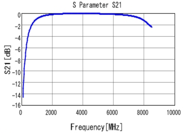
■ GRM1885C1H3R0CA01 S21 DCOV, 25degC
