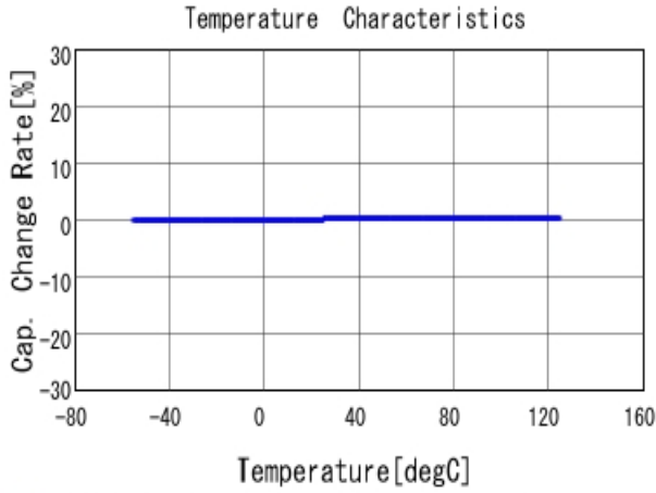
■ GRM1885C1H3R0CA01 C-Temp. capchange, DCOV, AC1Vrms
