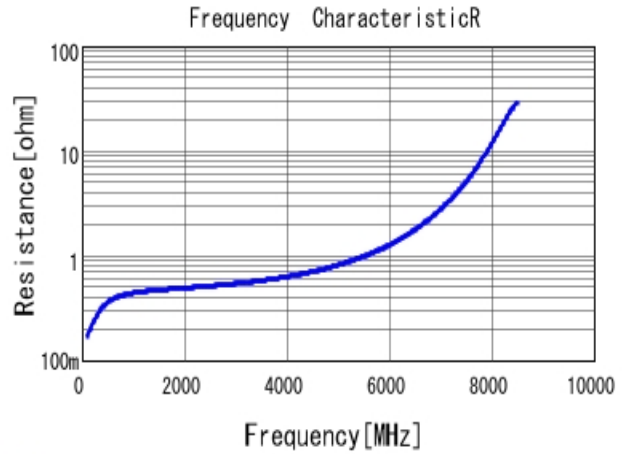
■ GRM1885C1H3R0CA01 R DC0V, 25degC
