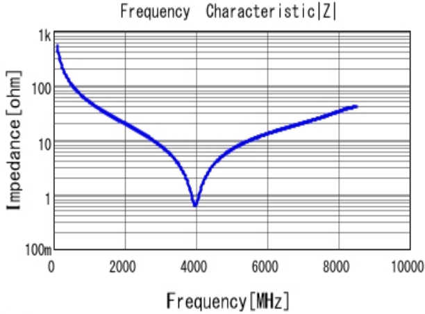
■ GRM1885C1H3R0BA01 |Z| DC0V, 25degC
