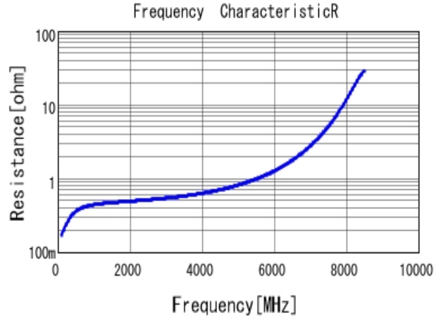
■ GRM1885C1H3R0BA01 R DC0V, 25degC
