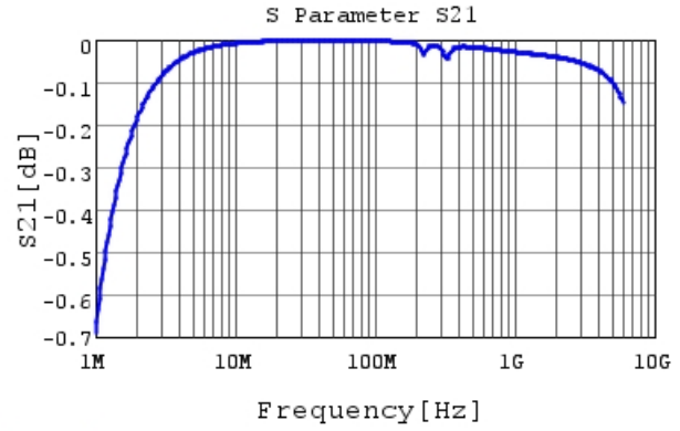
GRM1885C1H392JA01 S21 DCOV, 25degC
