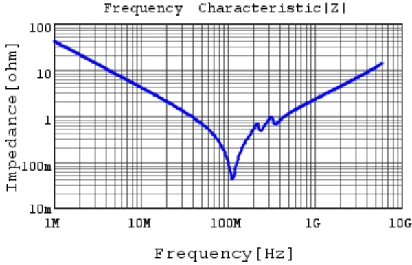
GRM1885C1H392JA01 |Z| DCOV, 25degC
