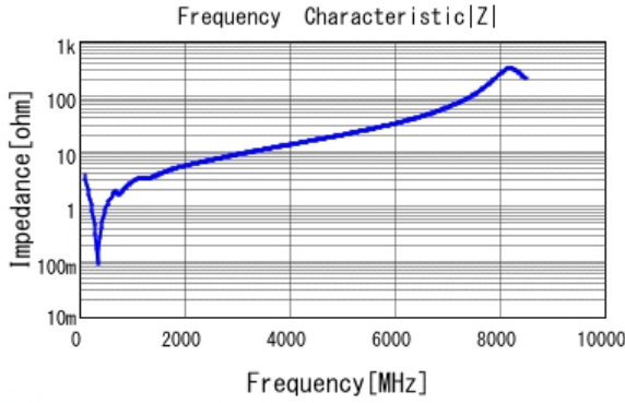
■ GRM1885C1H391JA01 |Z| DCOV, 25degC
