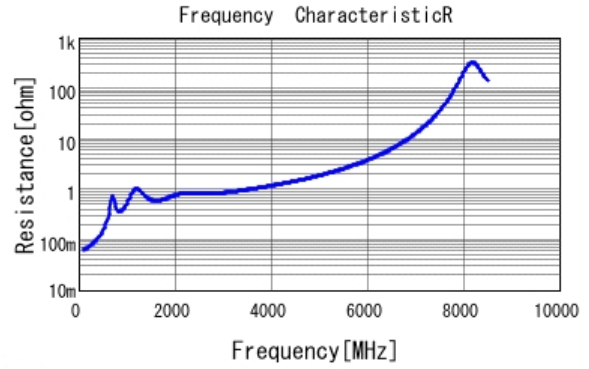
■ GRM1885C1H391JA01 R DCOV, 25degC
