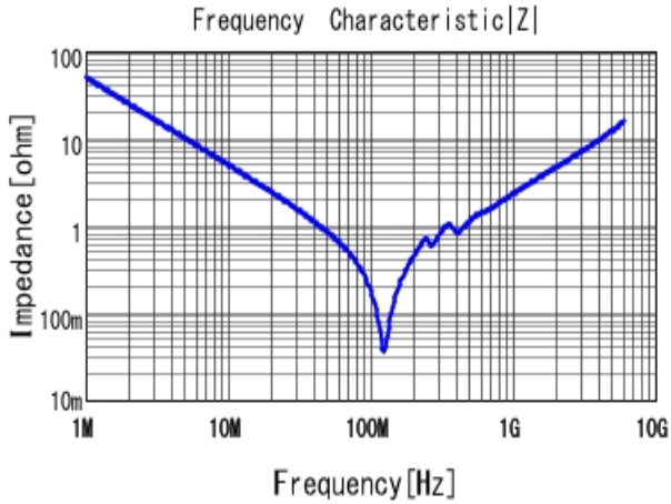
■ GRM1885C1H332JA01 |Z| DCOV, 25degC
