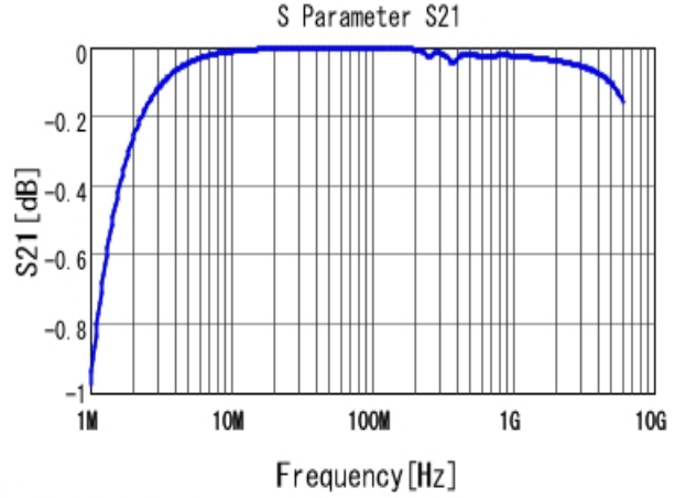
■ GRM1885C1H332JA01 S21 DCOV, 25degC
