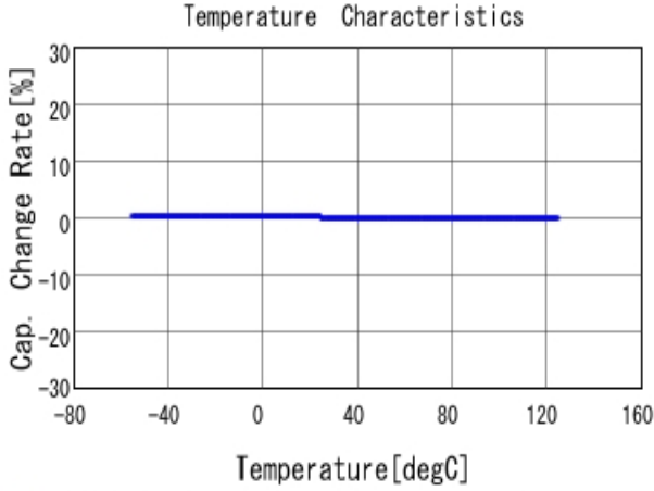
■ GRM1885C1H332JA01 C-Temp. capchange, DCOV, AC1Vrms
