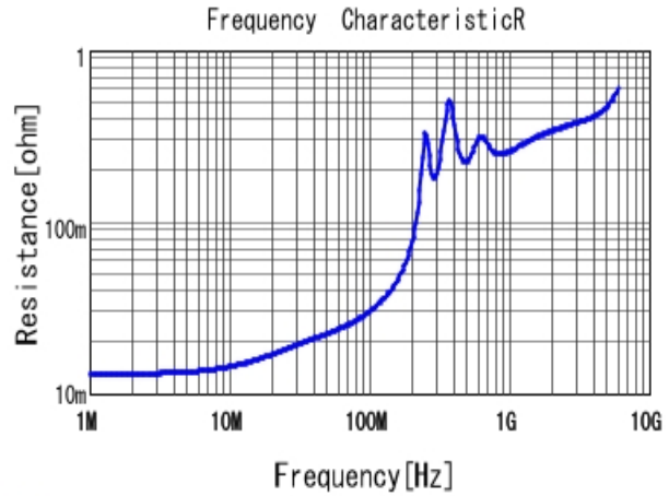
■ GRM1885C1H332JA01 R DCOV, 25degC
