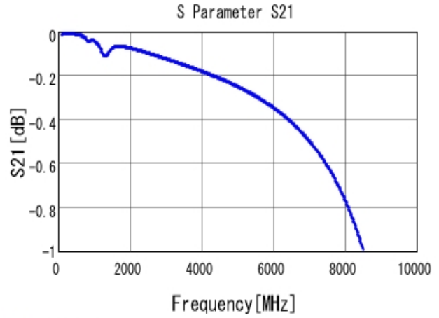
■ GRM1885C1H331JA01 S21 DCOV, 25degC
