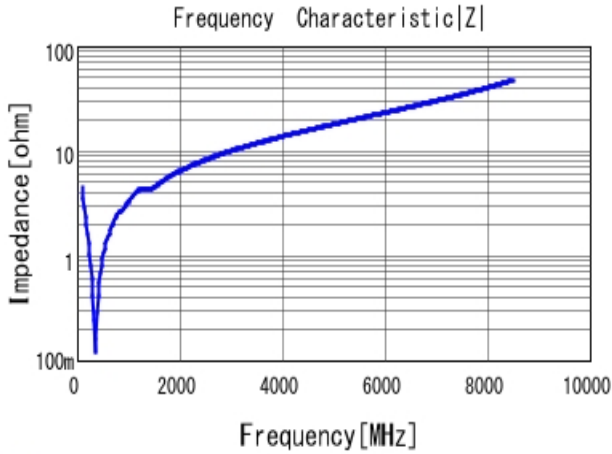
■ GRM1885C1H331JA01 |Z| DCOV, 25degC
