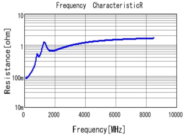
■ GRM1885C1H331JA01 R DCOV, 25degC
