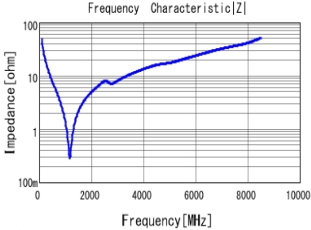
■ GRM1885C1H330JA01 |Z| DCOV, 25degC
