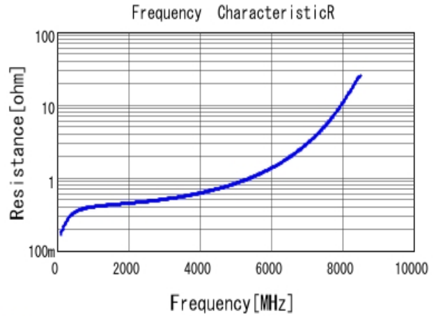
■ GRM1885C1H2R7CA01 R DCOV, 25degC
