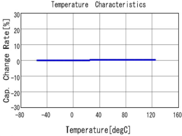
■ GRM1885C1H2R7CA01 C-Temp. capchange, DCOV, AC1Vrms
