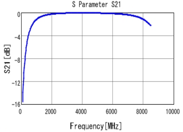
■ GRM1885C1H2R7CA01 S21 DCOV, 25degC
