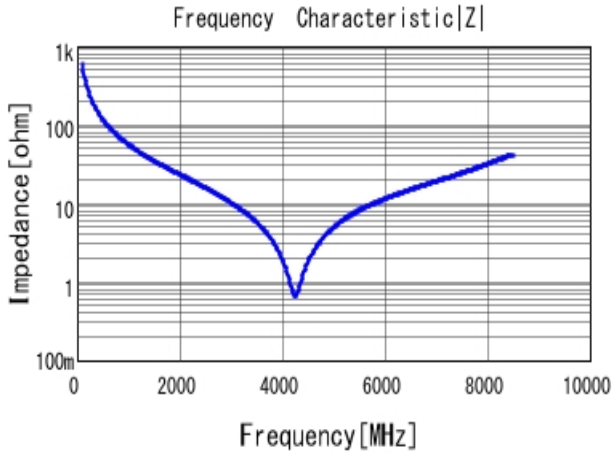
■ GRM1885C1H2R7CA01 |Z| DCOV, 25degC
