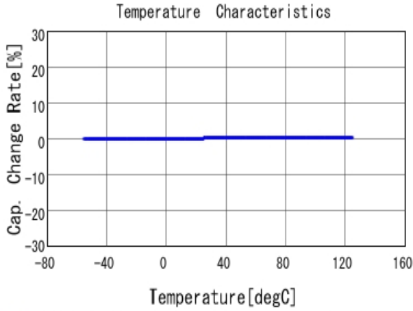
■ GRM1885C1H2R0BA01 C-Temp. capchange, DCOV, AC1Vrms
