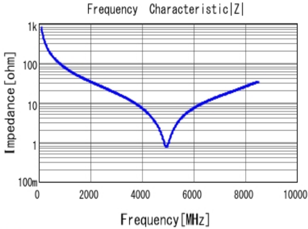
■ GRM1885C1H2R0BA01 |Z| DCOV, 25degC
