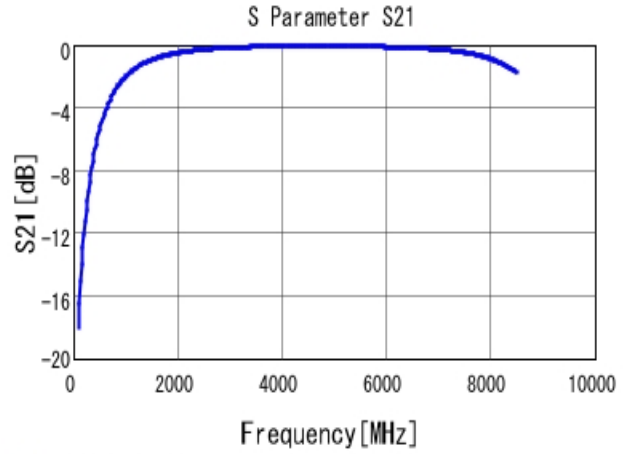
■ GRM1885C1H2R0BA01 S21 DCOV, 25degC
