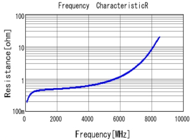
■ GRM1885C1H2R0BA01 R DCOV, 25degC
