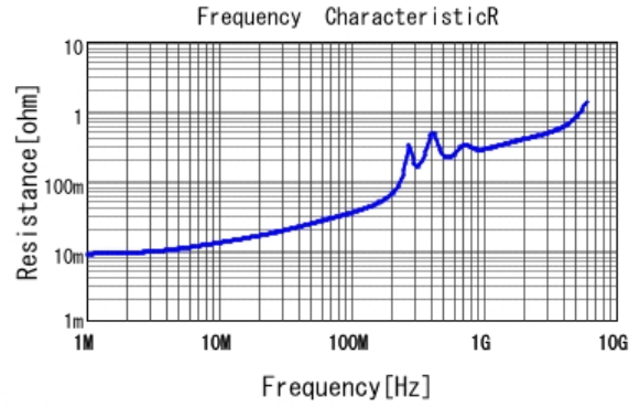
■ GRM1885C1H272JA01 R DCOV, 25degC
