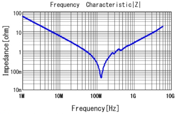
■ GRM1885C1H272JA01 |Z| DCOV, 25degC
