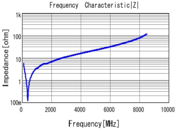
■ GRM1885C1H271JA01 |Z| DCOV, 25degC
