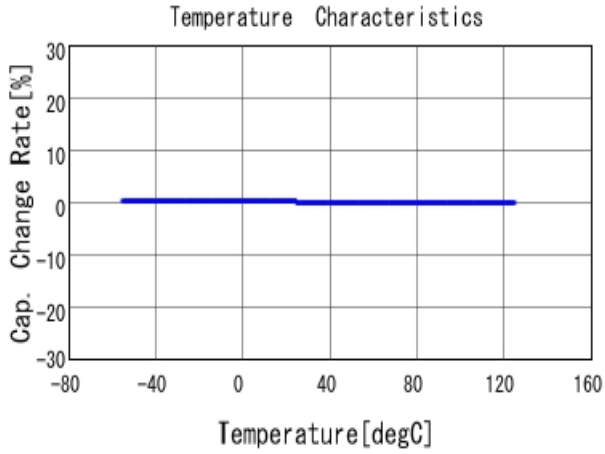
■ GRM1885C1H271JA01 C-Temp. capchange, DCOV, AC1Vrms
