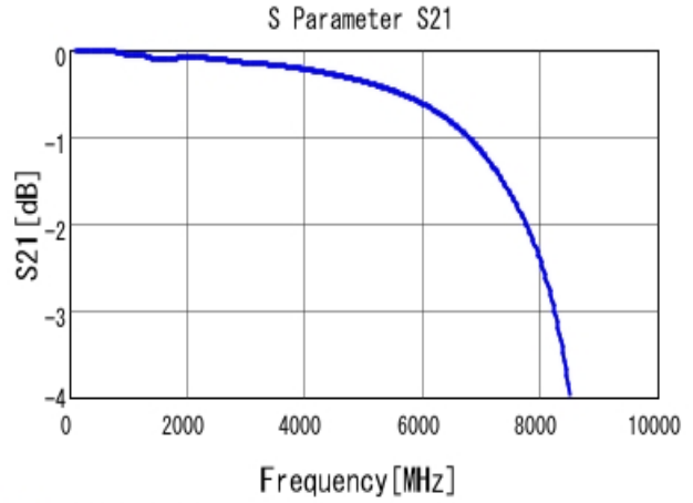
■ GRM1885C1H271JA01 S21 DCOV, 25degC
