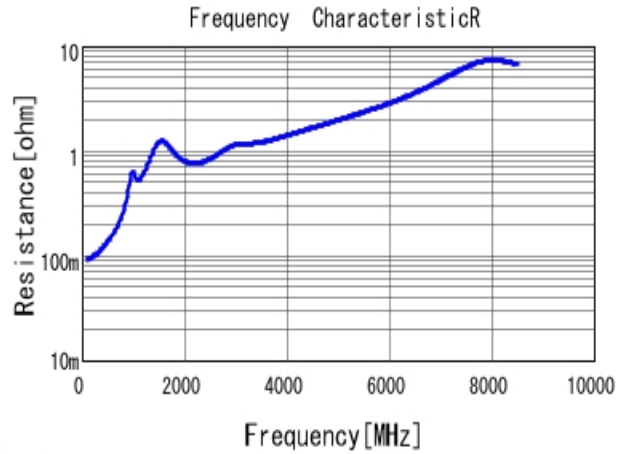
■ GRM1885C1H271JA01 R DCOV, 25degC
