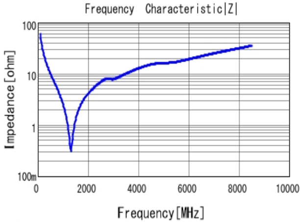
■ GRM1885C1H270JA01 |Z| DC0V, 25degC
