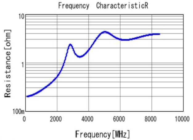
■ GRM1885C1H270JA01 R DC0V, 25degC
