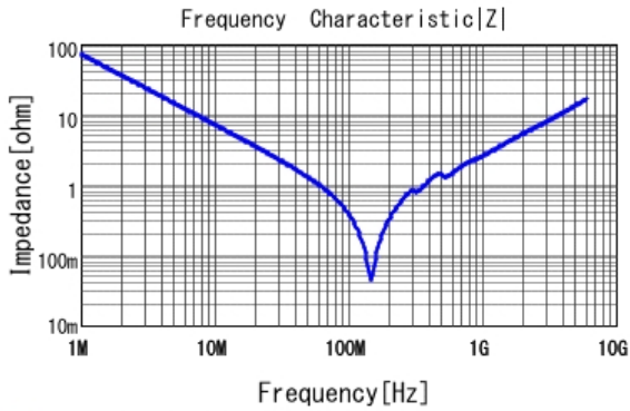
■ GRM1885C1H222JA01 |Z| DCOV, 25degC
