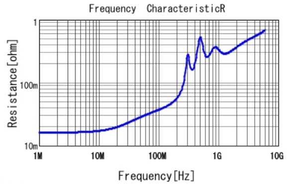
■ GRM1885C1H222JA01 R DCOV, 25degC
