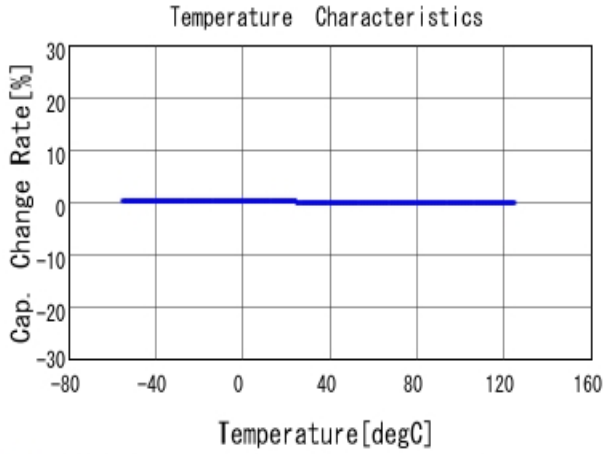
■ GRM1885C1H221JA01 C-Temp. capchange, DCOV, AC1Vrms
