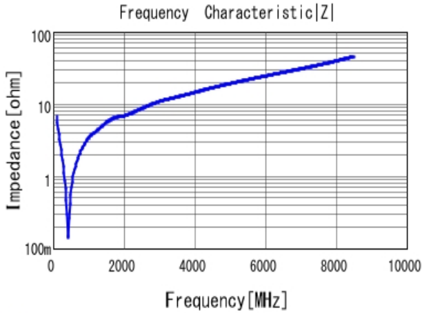
■ GRM1885C1H221JA01 |Z| DCOV, 25degC
