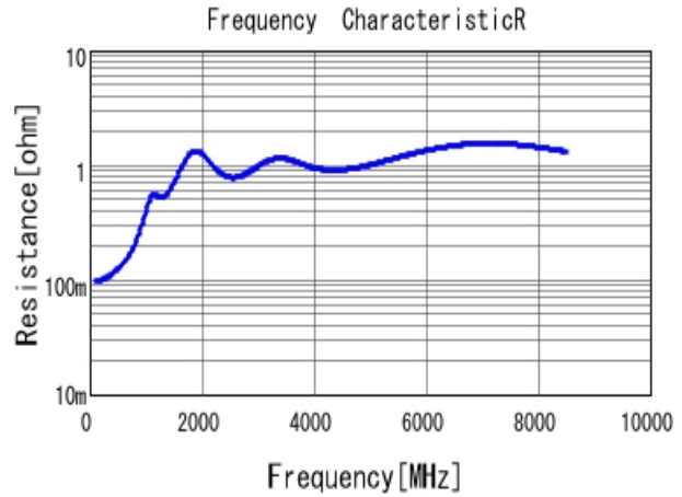
■ GRM1885C1H221JA01 R DCOV, 25degC
