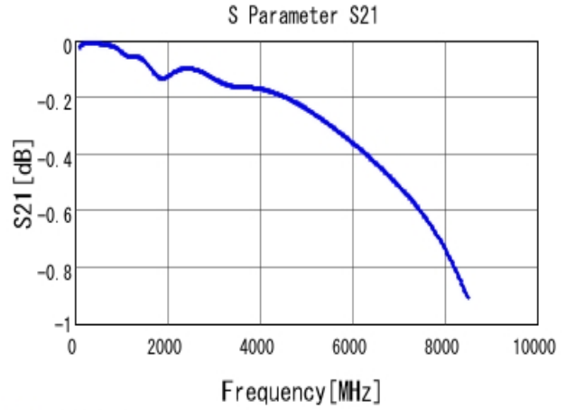
■ GRM1885C1H221JA01 S21 DCOV, 25degC
