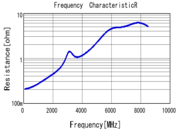
■ GRM1885C1H220JA01 R DCOV, 25degC
