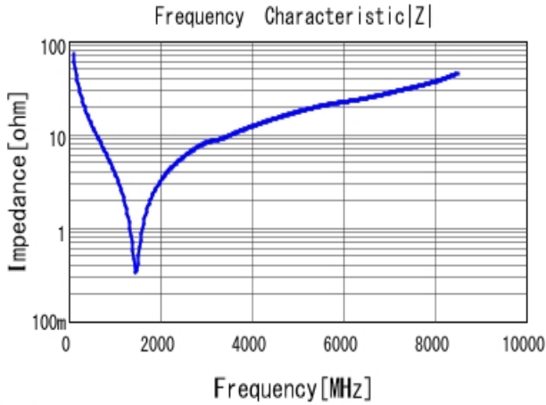
■ GRM1885C1H220JA01 |Z| DCOV, 25degC
