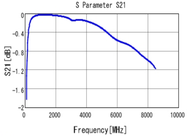
■ GRM1885C1H220JA01 S21 DCOV, 25degC
