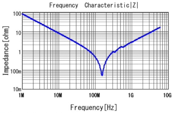
■ GRM1885C1H202JA01 |Z| DCOV, 25degC
