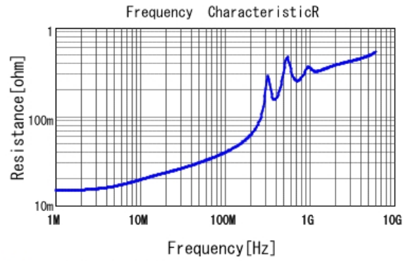
■ GRM1885C1H202JA01 R DCOV, 25degC
