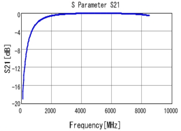
■ GRM1885C1H1R8CA01 S21 DCOV, 25degC
