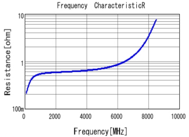
■ GRM1885C1H1R6CA01 R DCOV, 25degC
