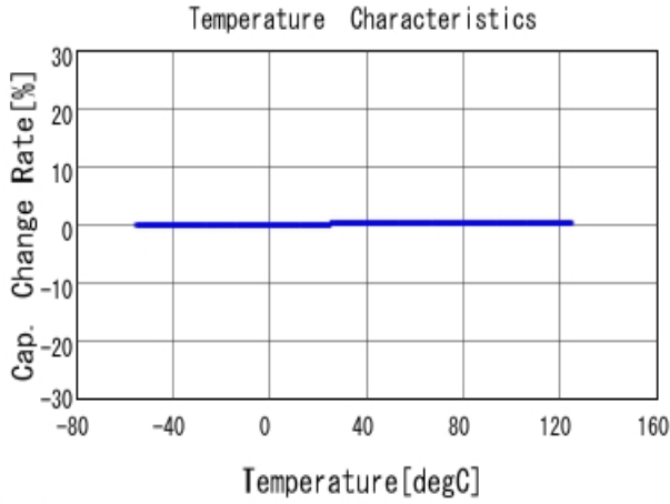
■ GRM1885C1H1R6CA01 C-Temp. capchange, DCOV, AC1Vrms
