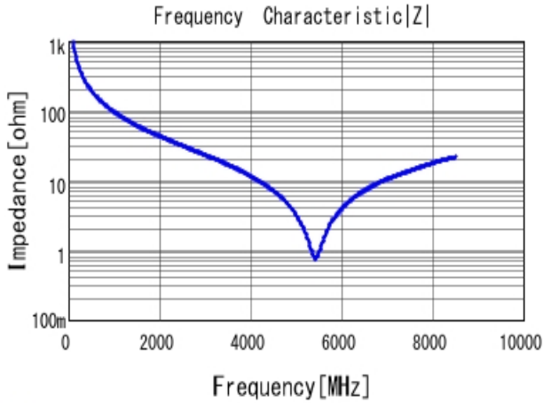
■ GRM1885C1H1R6CA01 |Z| DCOV, 25degC
