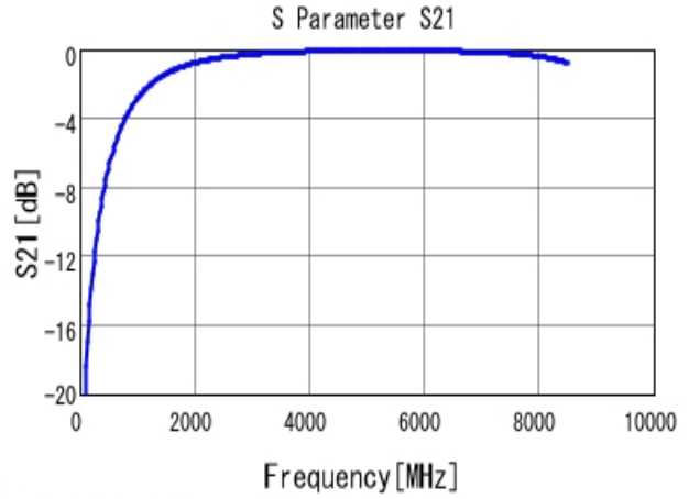
■ GRM1885C1H1R6CA01 S21 DCOV, 25degC
