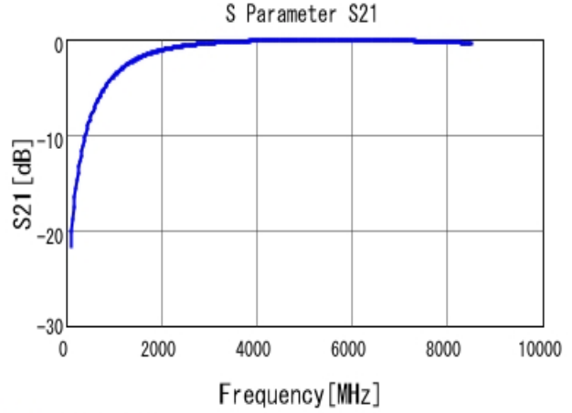
■ GRM1885C1H1R3CA01 S21 DCOV, 25degC
