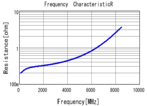
■ GRM1885C1H1R3CA01 R DCOV, 25degC
