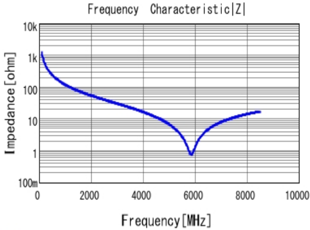
■ GRM1885C1H1R3CA01 |Z| DCOV, 25degC
