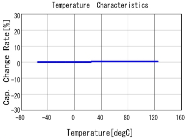
■ GRM1885C1H1R2CA01 C-Temp. capchange, DCOV, AC1Vrms
