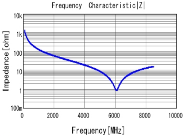
■ GRM1885C1H1R2CA01 |Z| DCOV, 25degC
