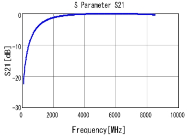
■ GRM1885C1H1R2CA01 S21 DCOV, 25degC
