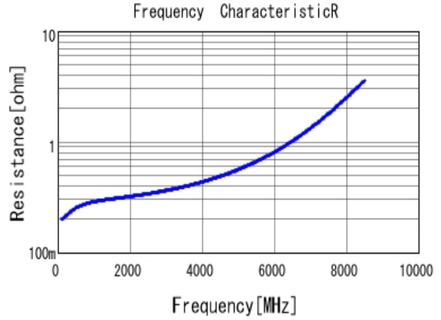
■ GRM1885C1H1R2BA01 R DCOV, 25degC
