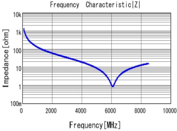
■ GRM1885C1H1R2BA01 |Z| DCOV, 25degC
