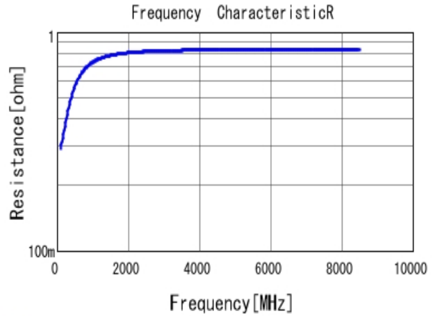
■ GRM1885C1H1R0WA01 R DCOV, 25degC
