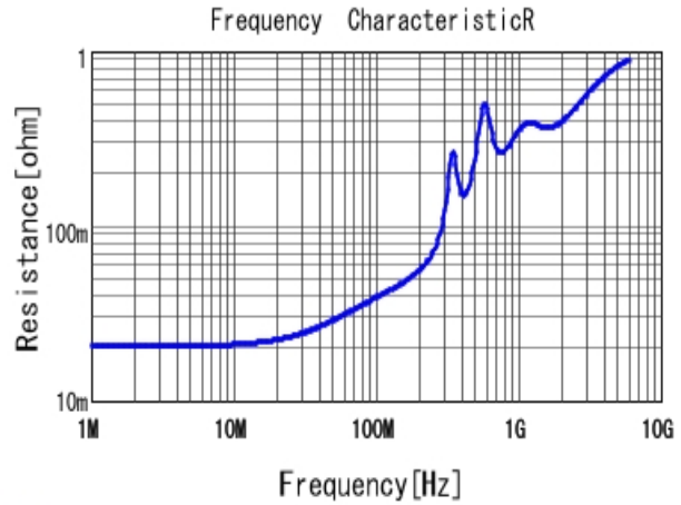
■ GRM1885C1H182JA01 R DCOV, 25degC
