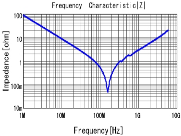
■ GRM1885C1H182JA01 |Z| DCOV, 25degC
