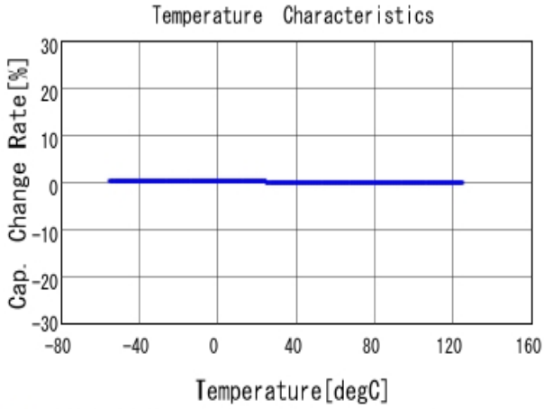
■ GRM1885C1H182JA01 C-Temp. capchange, DCOV, AC1Vrms
