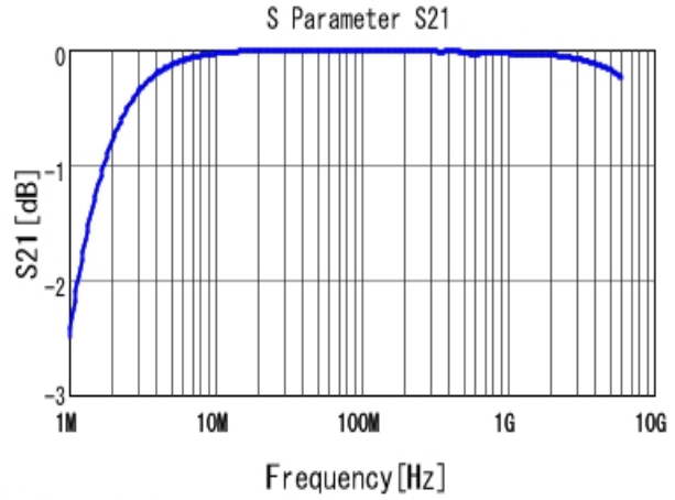
■ GRM1885C1H182JA01 S21 DCOV, 25degC
