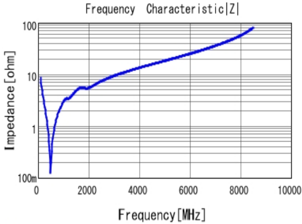
■ GRM1885C1H181JA01 |Z| DCOV, 25degC
