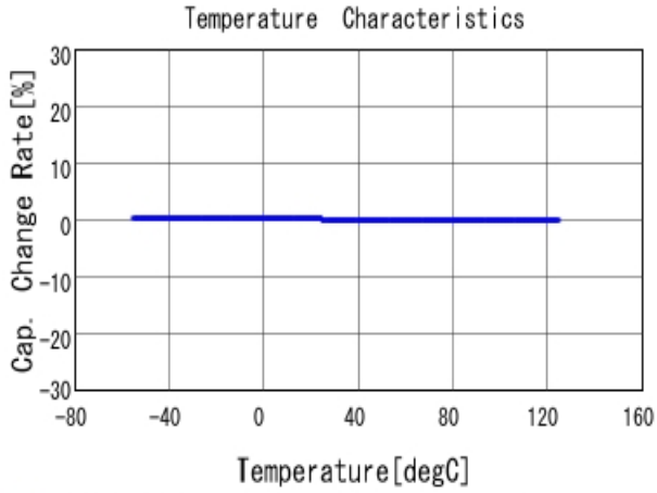
■ GRM1885C1H181JA01 C-Temp. capchange, DCOV, AC1Vrms
