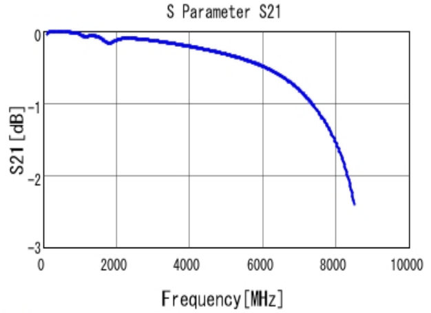
■ GRM1885C1H181JA01 S21 DCOV, 25degC
