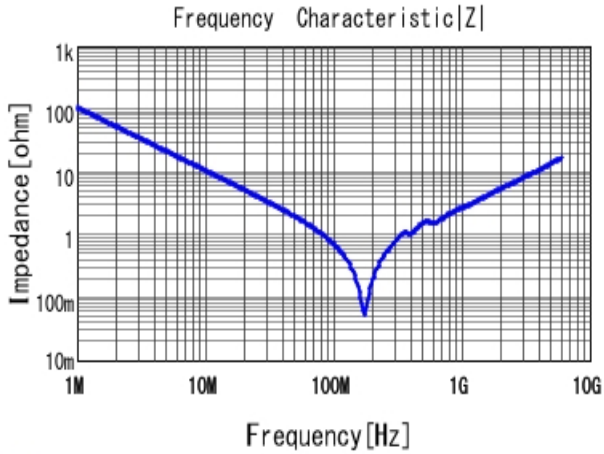
■ GRM1885C1H152JA01 |Z| DC0V, 25degC
