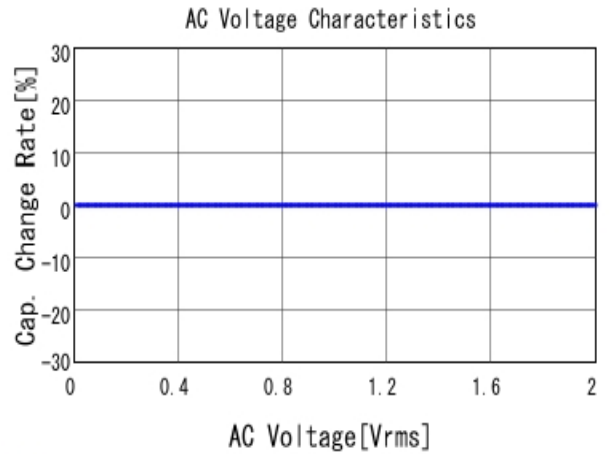
■ GRM1885C1H152JA01 C-AC Voltage capchange, DC0V, 25.0d
