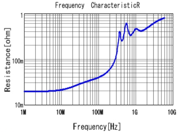
■ GRM1885C1H152JA01 R DC0V, 25degC
