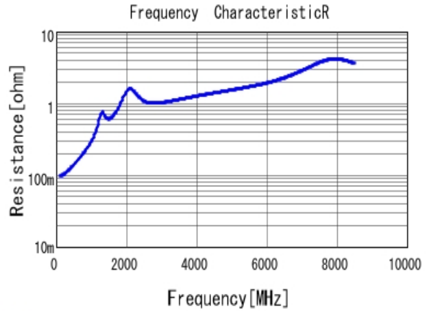
■ GRM1885C1H151JA01 R DCOV, 25degC
