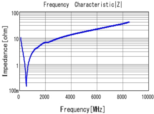
■ GRM1885C1H151JA01 |Z| DCOV, 25degC
