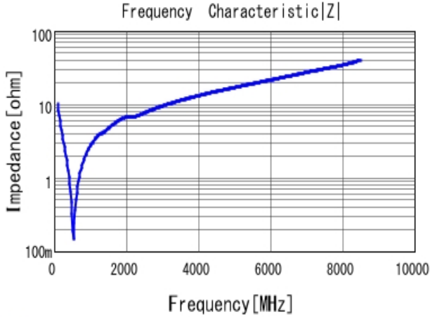
■ GRM1885C1H151GA01 |Z| DCOV, 25degC
