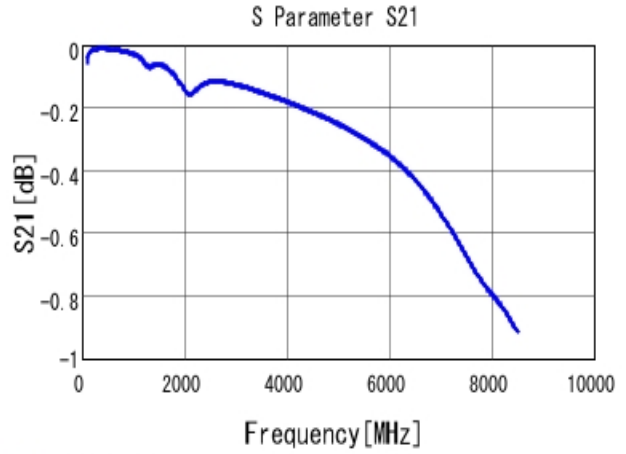
■ GRM1885C1H151GA01 S21 DCOV, 25degC
