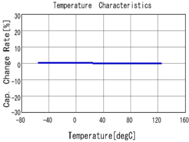
■ GRM1885C1H151GA01 C-Temp. capchange, DCOV, AC1Vrms
