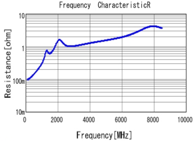
■ GRM1885C1H151GA01 R DCOV, 25degC
