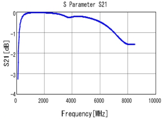
■ GRM1885C1H150JA01 S21 DCOV, 25degC
