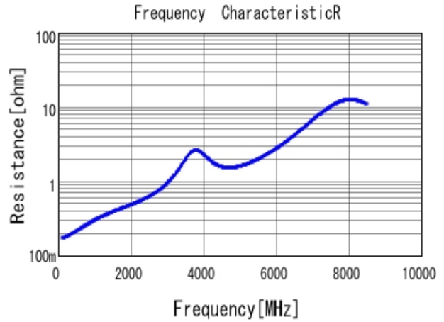
■ GRM1885C1H150JA01 R DCOV, 25degC
