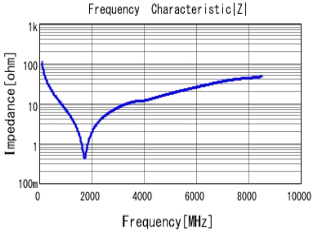
■ GRM1885C1H150JA01 |Z| DCOV, 25degC
