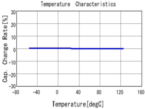
■ GRM1885C1H150JA01 C-Temp. capchange, DCOV, AC1Vrms
