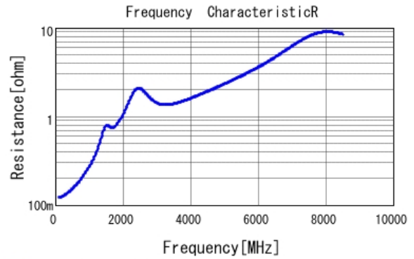
■ GRM1885C1H121JA01 R DCOV, 25degC
