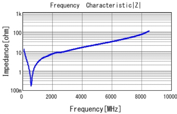
■ GRM1885C1H121JA01 |Z| DCOV, 25degC
