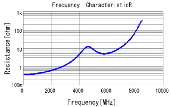
■ GRM1885C1H120JA01 R DCOV, 25degC
