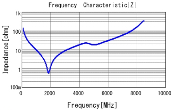
■ GRM1885C1H120JA01 |Z| DCOV, 25degC
