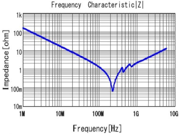
■ GRM1885C1H102JA01 |Z| DCOV, 25degC
