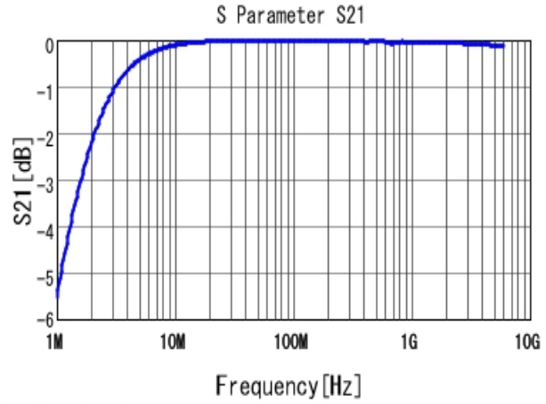
■ GRM1885C1H102JA01 S21 DCOV, 25degC
