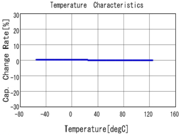
■ GRM1885C1H102JA01 C-Temp. capchange, DCOV, AC1Vrms
