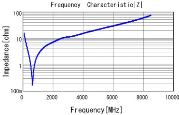
■ GRM1885C1H101JA01 |Z| DCOV, 25degC
