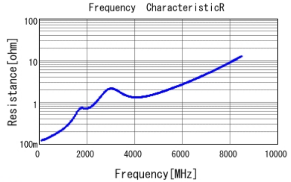
■ GRM1885C1H101JA01 R DCOV, 25degC
